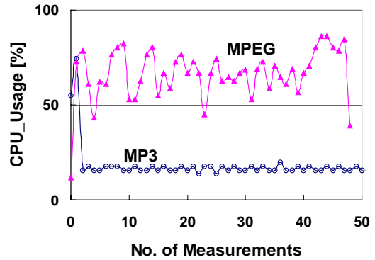
Fig. 2. CPU usage of MP3 and MPEG
