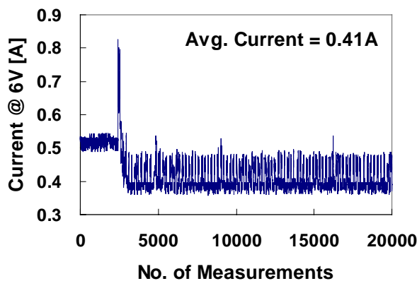
Fig. 13. Power consumption with DVFS at fps=1
