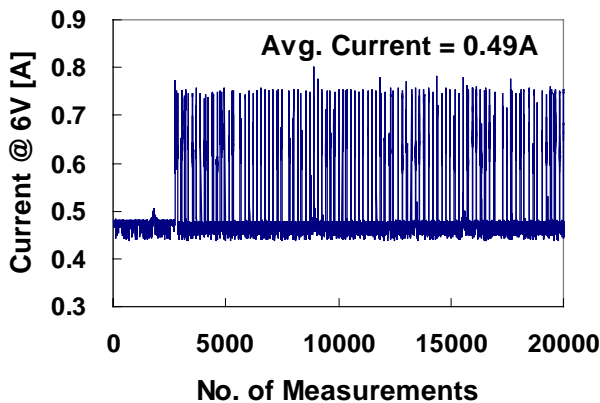
Fig. 12. Power consumption without DVFS at fps=1
