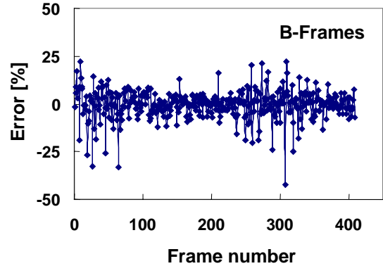
Fig. 7. Errors in B-frame workload prediction
