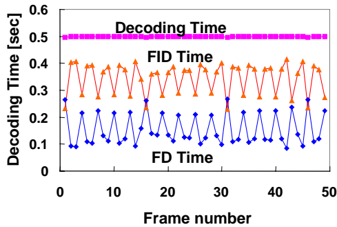
Fig. 5. Decoding time with fps = 2
