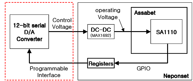
Fig. 10. Variable voltage generator for the test bed
