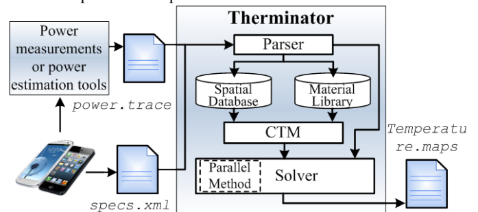
Figure 1. Overview of Therminator.
