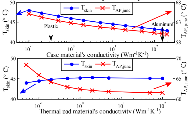
Figure 9. Skin and AP junction temperature versus rear case material (a) and thermal pad material (b) for P_{AP} = 2.2W .
