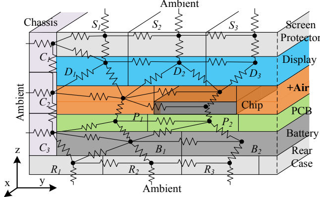
Figure 2. A cross-section view of the thermal resistance network in a simple smartphone model.
